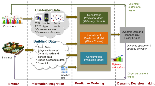
Figure 2: D2R Framework
